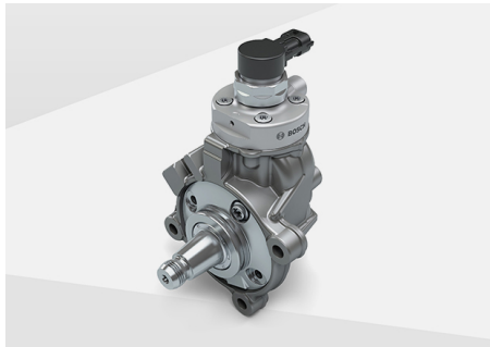
Single plunger high-pressure pump CP4-25/1 E with electric suction valve
